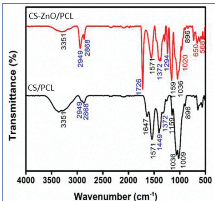
[Table/Fig-8]: FTIR spectra of the bi-layered scaffold with peaks indicating the presence of PCL, Chitosan, and Zinc oxide, and suggestive of the interactions between PCL and ZnO.
